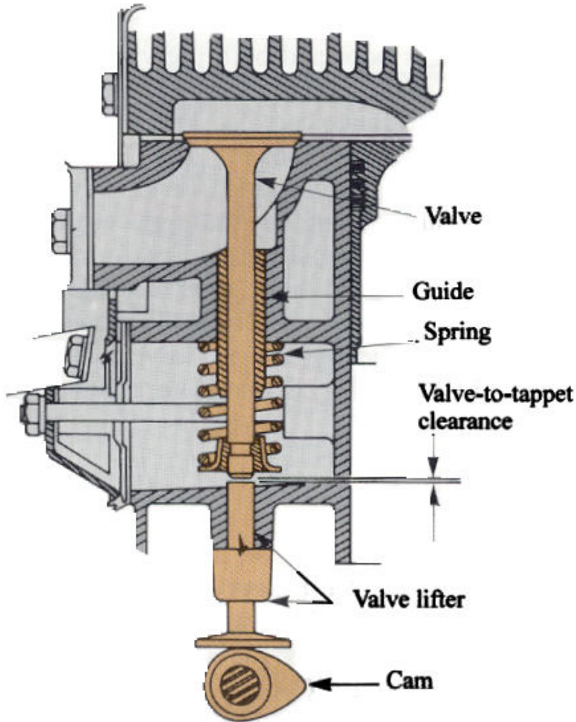
Figure 17-61. Components of a complete valve train. (Kohler Co.)
