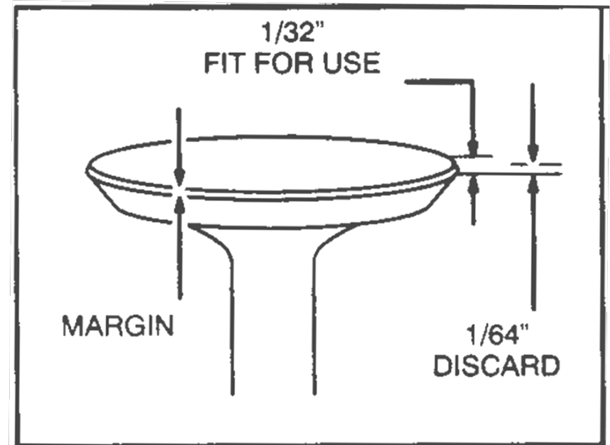
Fig. 6 - Valve and Seat Dimensions
