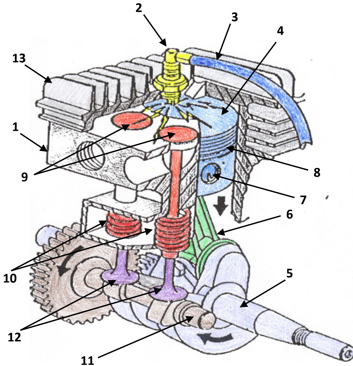
Parts of the 4-stroke Engine
